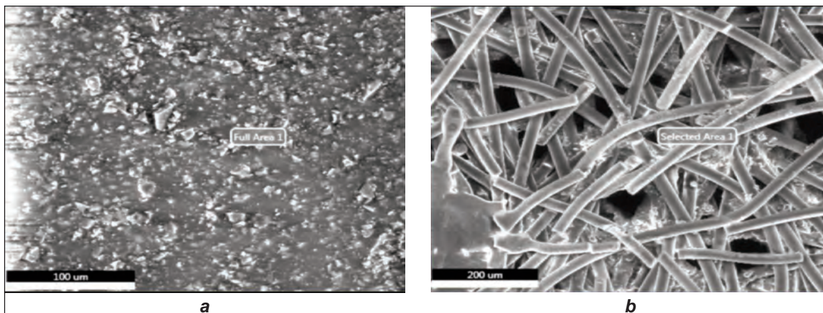
Fig. 8. Results of: a – EDS images of B-N1-5 at 100 μm; b – B-N1-5 at 200 μm samples
