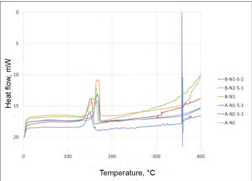
Fig. 6. Differential Scanning Calorimetry test results of fabric samples labelled A-N1-5, A-N2-5, B-N1-5, B-N2-5, A-N1, and B-N1
