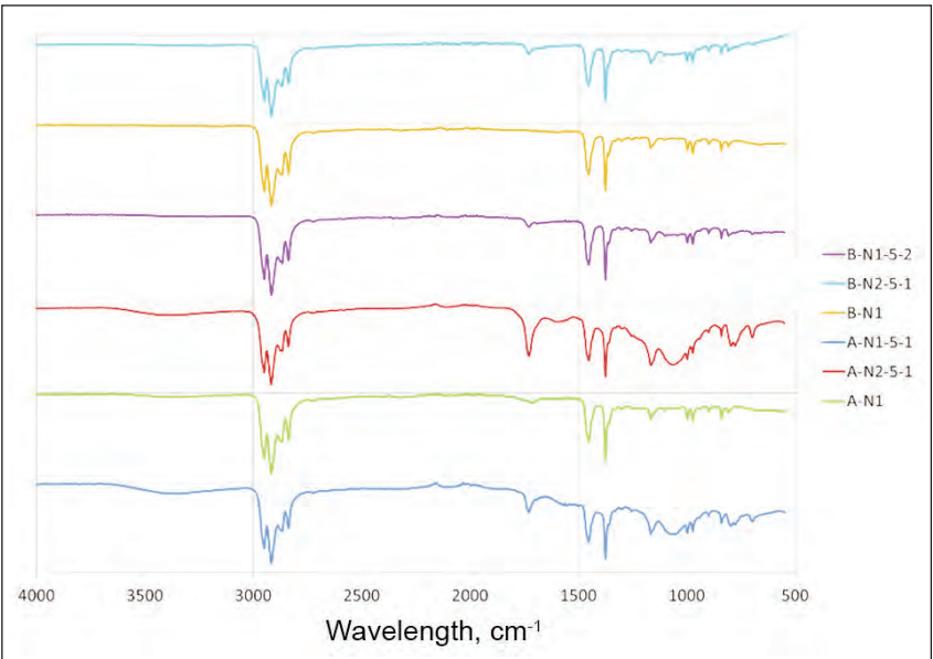
Fig. 5. FTIR test findings for non-woven fabric samples B-N1, B-N1-5-1, B-N2-5-1, A-N1, A-N1-5-1, A-N2-5-1
