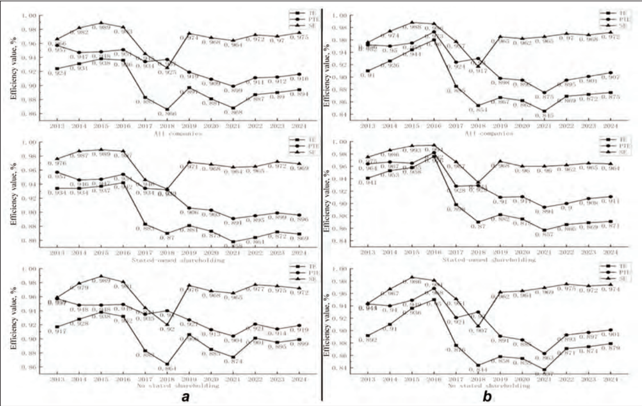
Fig. 2. Average technological innovation efficiency over the years: a – the first-stage DEA-BCC model; b – the second-stage DEA-BCC model
