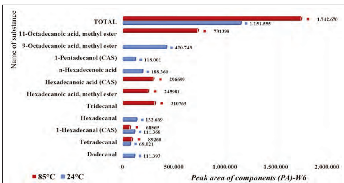
Fig. 9. GC-MS results of TF washed according to prescription code W6
