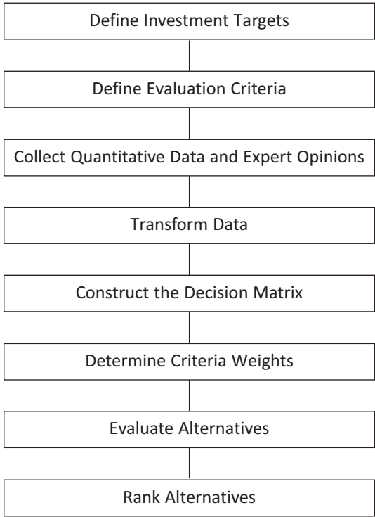
Fig. 1. Workflow diagram of the proposed linguistic MCDM method for machinery selection
