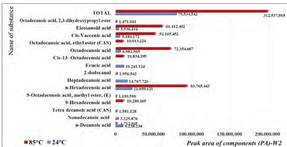
Fig. 5. GC-MS results of TF washed according to prescription code W2
