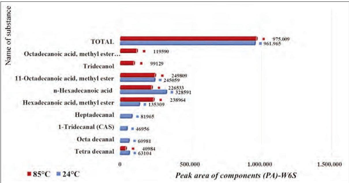
Fig. 14. GC-MS results of TFs washed according to the W6S code prescription
