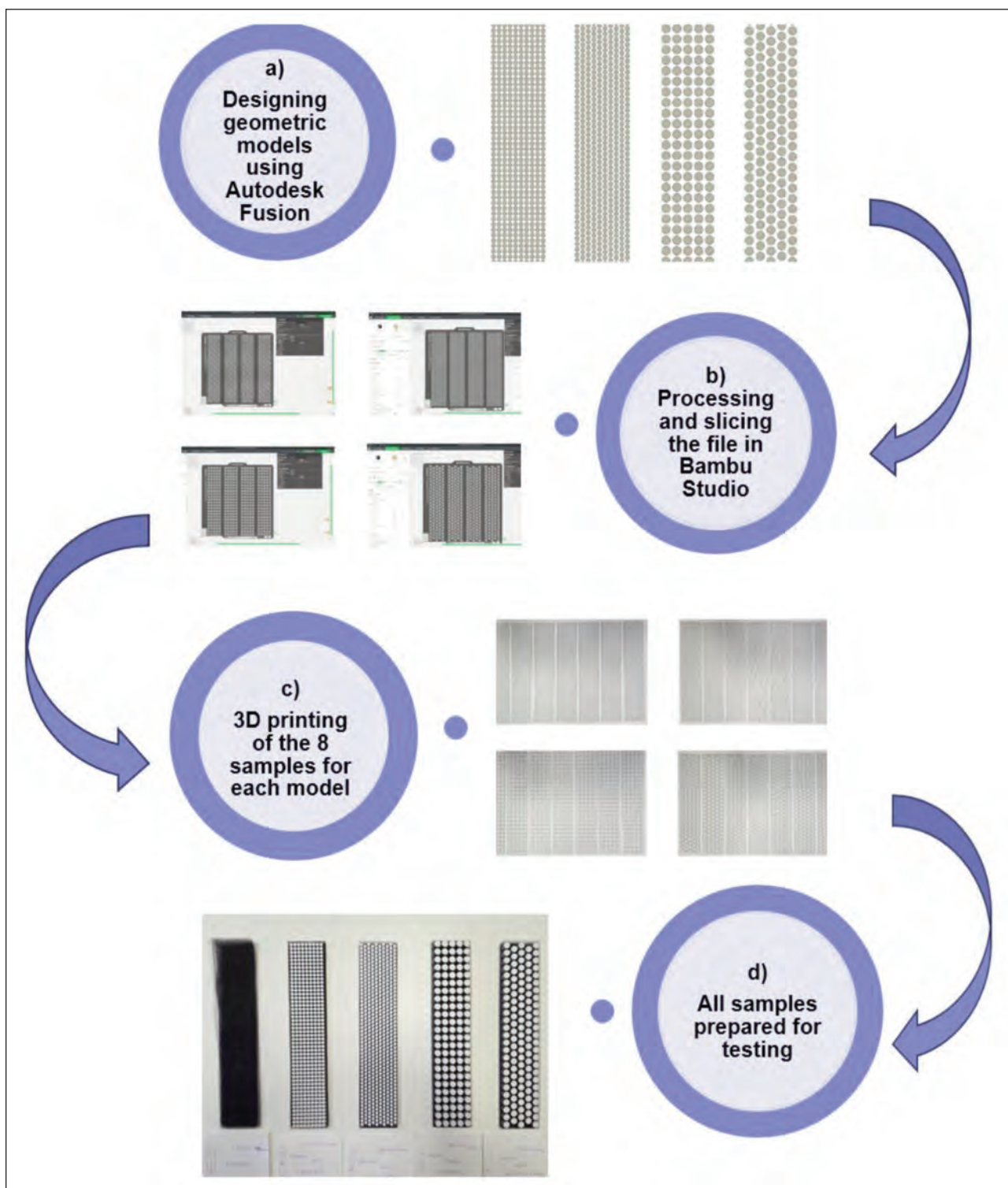
Fig. 2. The stages of making test samples
