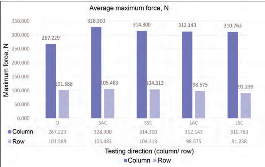
Fig. 6. Average Maximum force (N) depending on the testing direction
