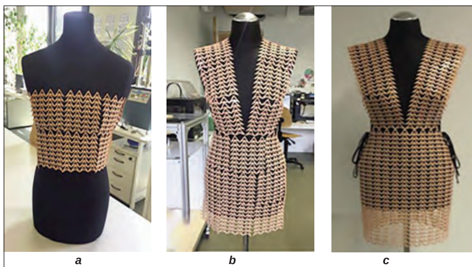
Fig. 6. Images of: a – 3D printed parts assembled by needle stitched on a mannequin; b – the whole dress; c – the finished dress with belts on both sides
