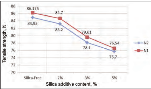
Fig. 2. Tensile strength outcomes of untreated, 2%, 3%, and 5% silica-modified polypropylene fabrics
