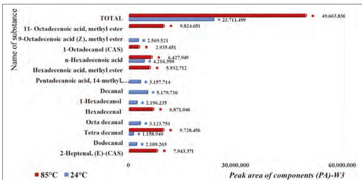
Fig. 6. GC-MS results of TF washed according to W3-coded prescription
