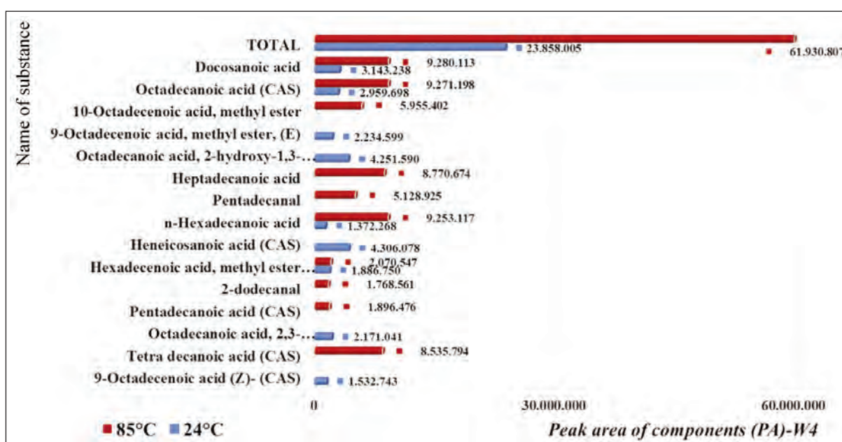
Fig. 7. GC-MS results of TF washed according to prescription code W4
