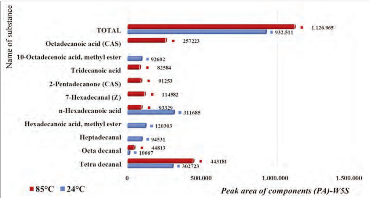
Fig. 13. GC-MS results of TFs washed according to the W5S-coded prescription
