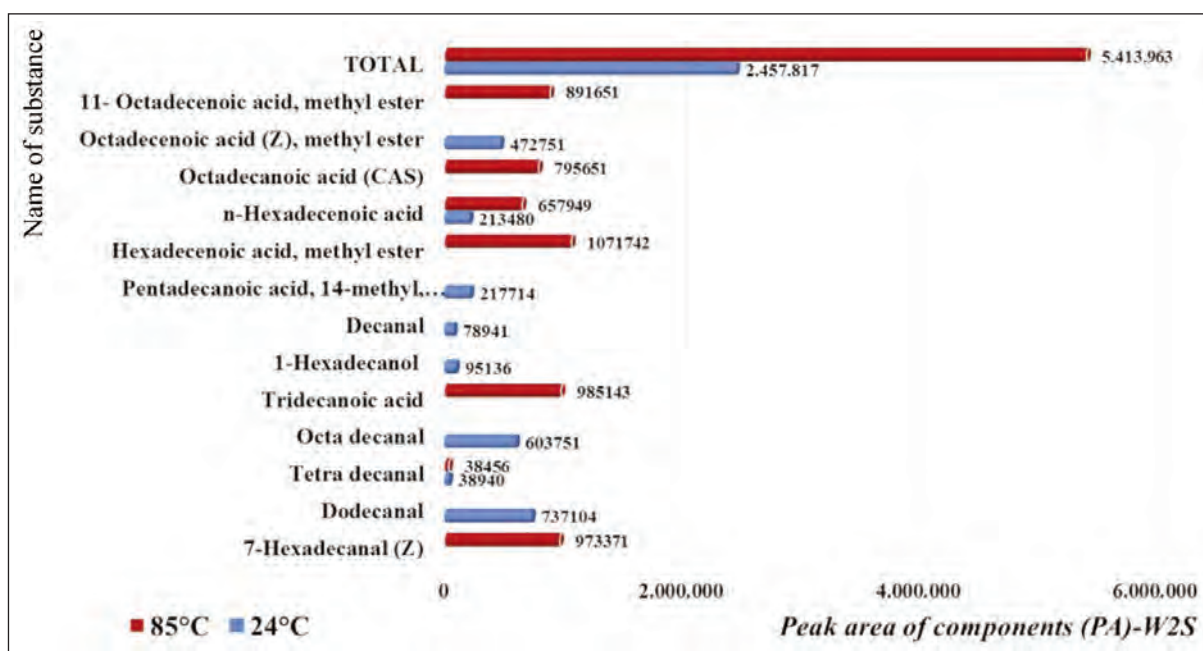
Fig. 10. GC-MS results of TFs washed according to the W2S-coded prescription
