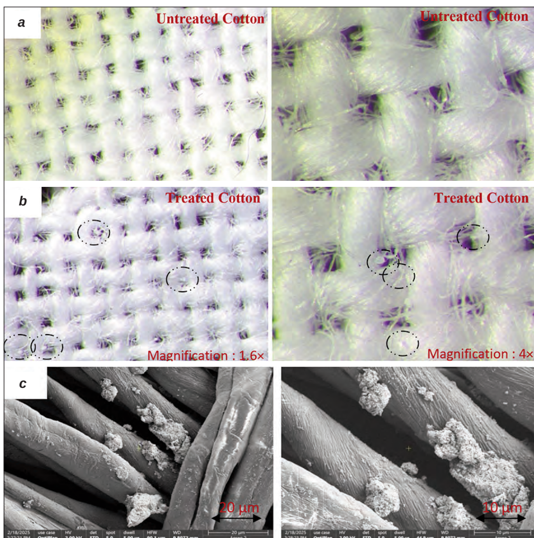
Fig. 5. Microscopic analysis comparing untreated and treated cotton fabric: a – optical micrograph of untreated fabric; b – optical micrograph of treated fabric; c – SEM images of treated fabric
