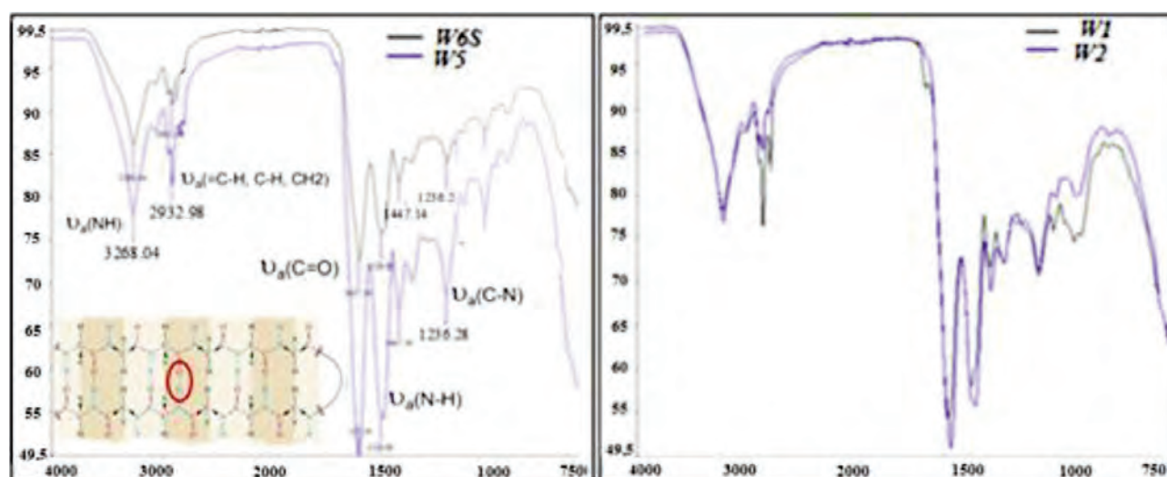
Fig. 3. FTIR spectra of TFs washed according to different washing methods
