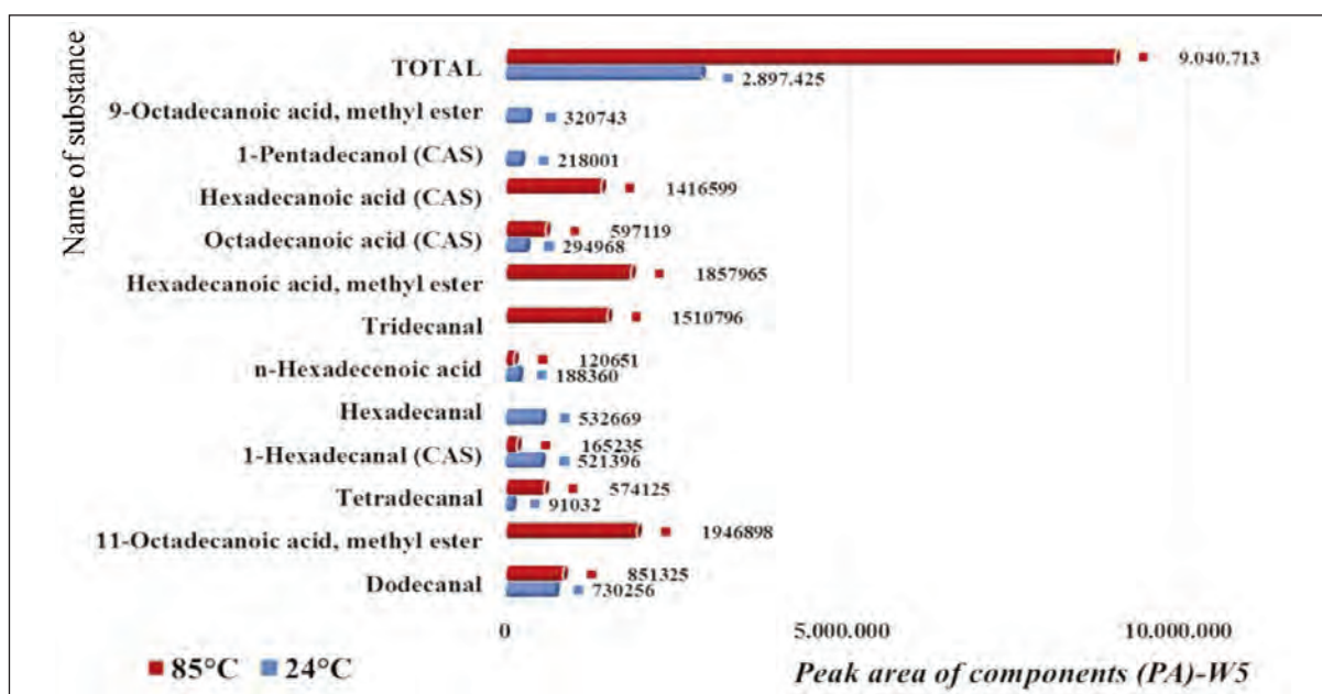
Fig. 8. GC-MS results of TF washed according to prescription code W5
