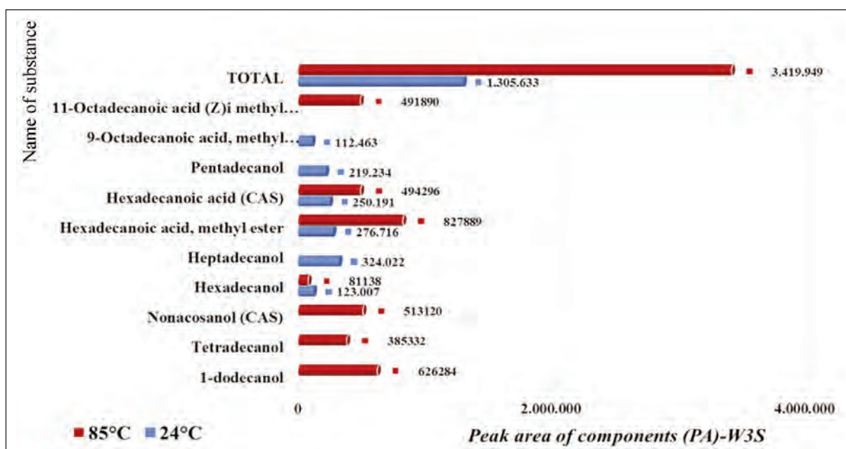
Fig. 11. GC-MS results of TFs washed according to the W3S-coded prescription
