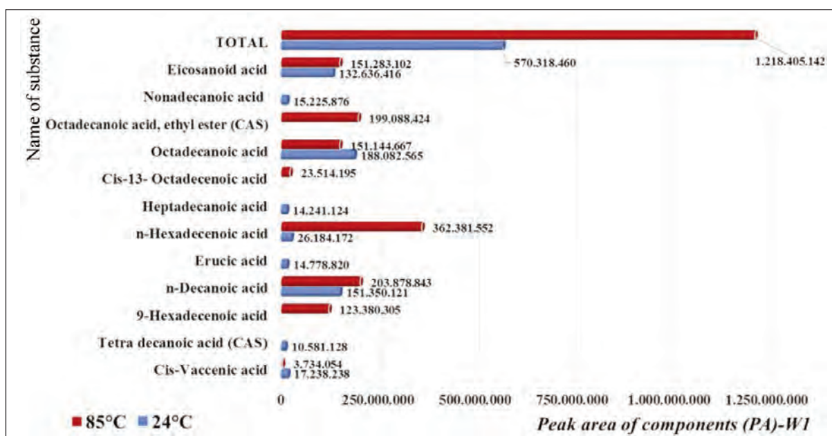
Fig. 4. GC-MS results of W1-coded TF rinsed in pure water
