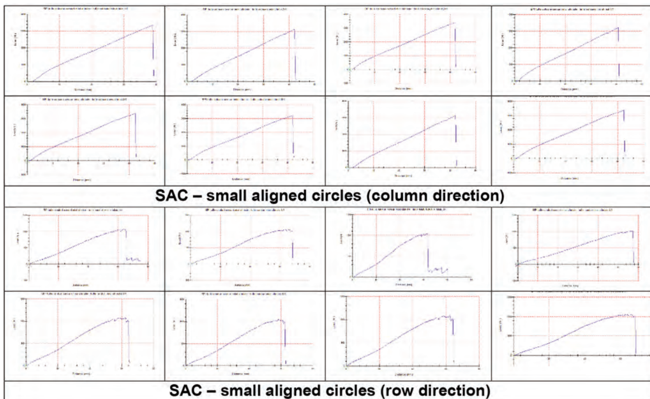
Fig. 9. The load-distance (force-extension) graphs for the SAC – Small Aligned Circles samples (column/ row direction)
