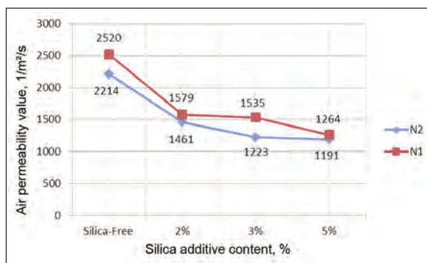
Fig. 1. Air permeability outcomes of untreated, 2%, 3%, and 5% silica-modified polypropylene fabrics
