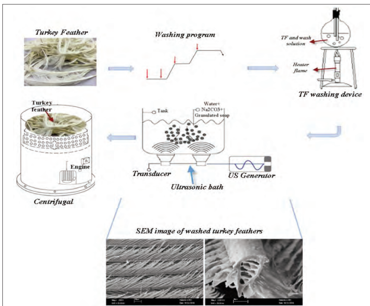
Fig. 1. Graphical summary of the TF washing process
