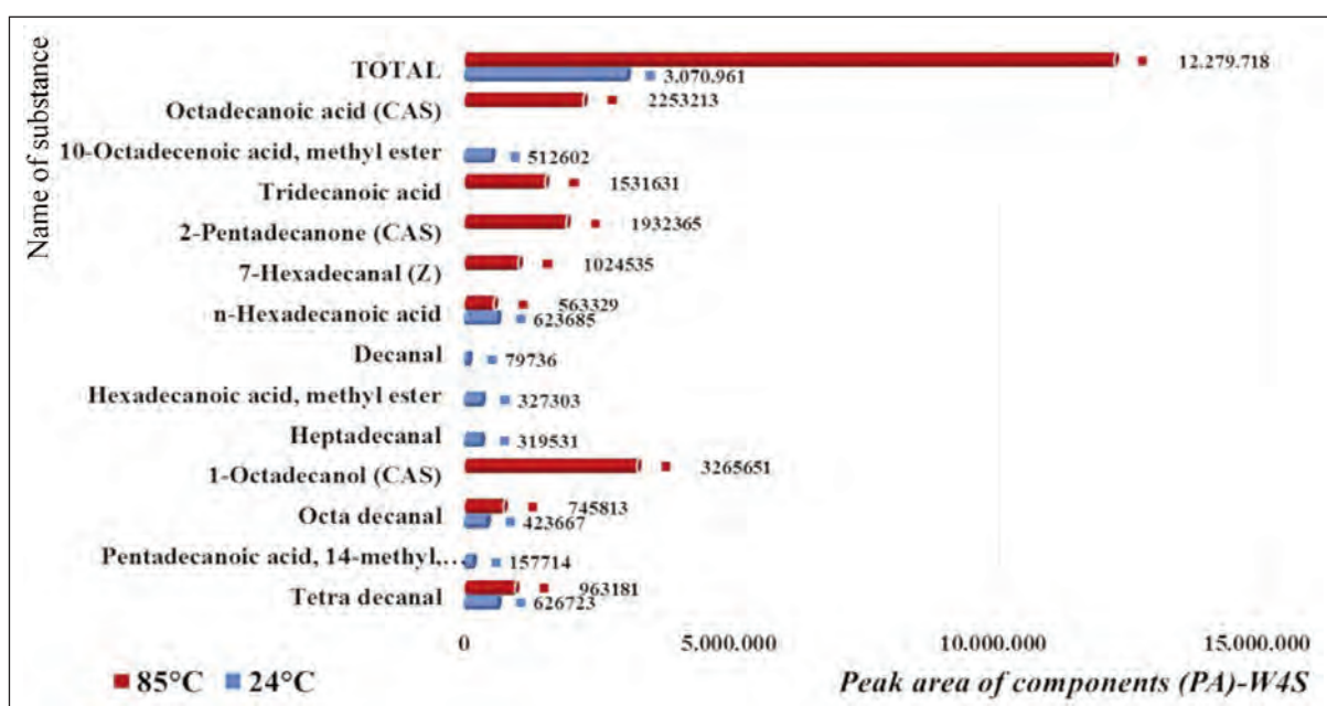
Fig. 12. GC-MS results of TFs washed according to the W4S code prescription
