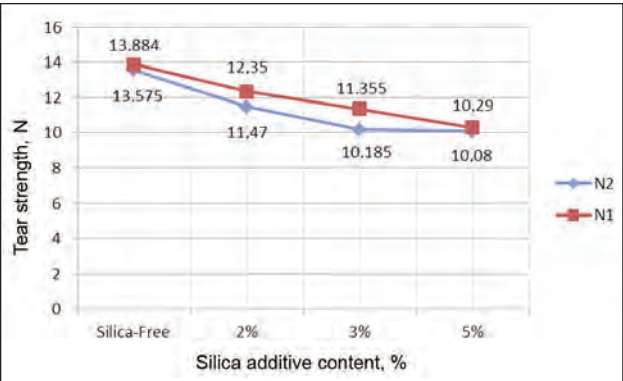
Fig. 3. Tear strength outcomes of untreated, 2%, 3%, and 5% silica-modified polypropylene fabrics
