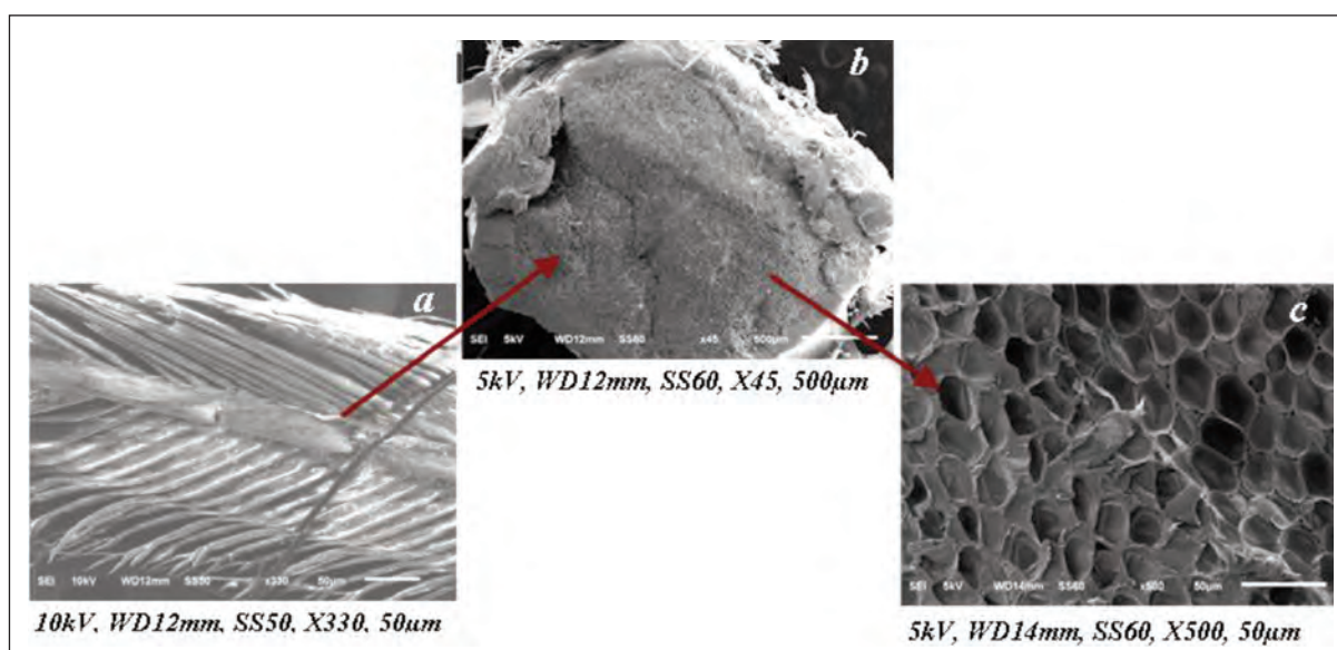
Fig. 2. SEM images of turkey feathers after washing: a – feather of turkey feather; b – rachis section; c – hollow internal structure of the feather
