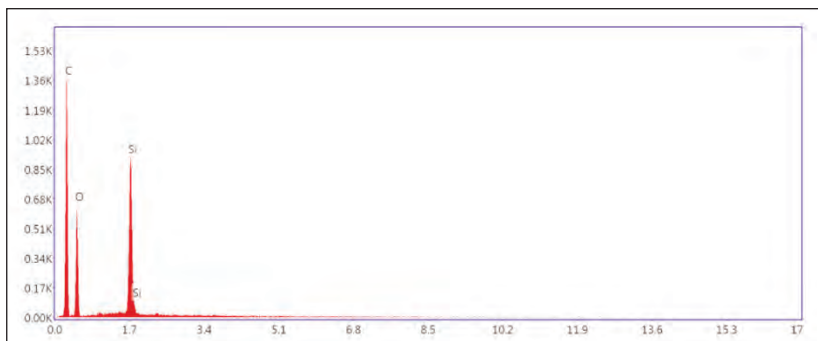
Fig. 10. EDS analysis results for sample B-N1-5
