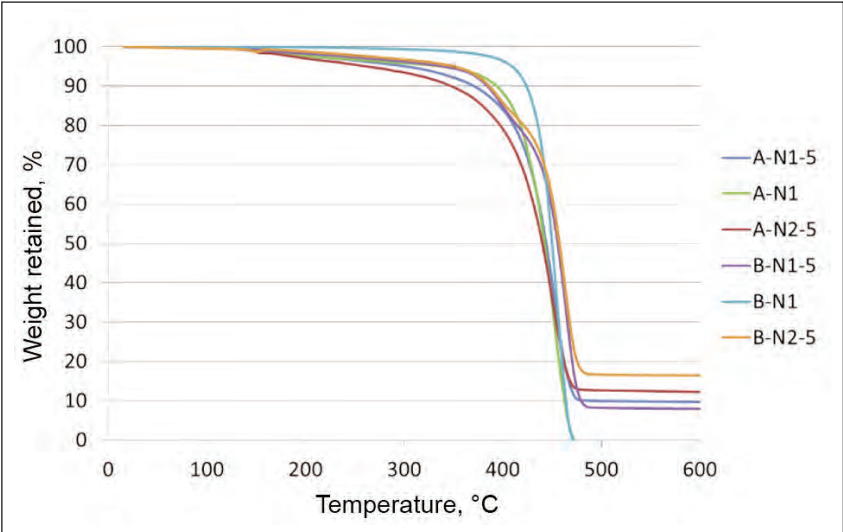
Fig. 7. The TGA test outcomes of fabric samples designated A-N1-5, A-N2-5, B-N1-5, B-N2-5, A-N1, and B-N1
