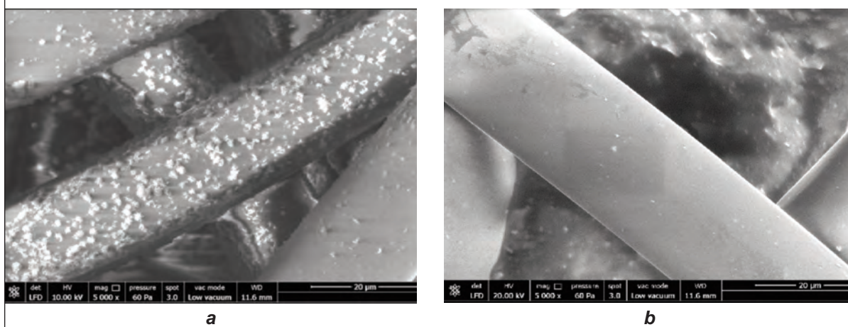
Fig. 9. Results of: a – SEM pictures of B-N1-5 at 20 μm; b – A-N1-5 at 20 μm samples
