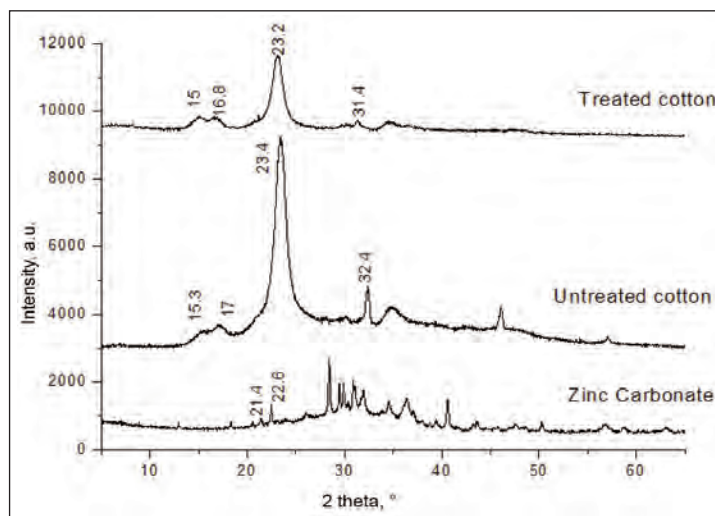
Fig. 3. XRD of zinc carbonate, untreated and treated cotton textile
