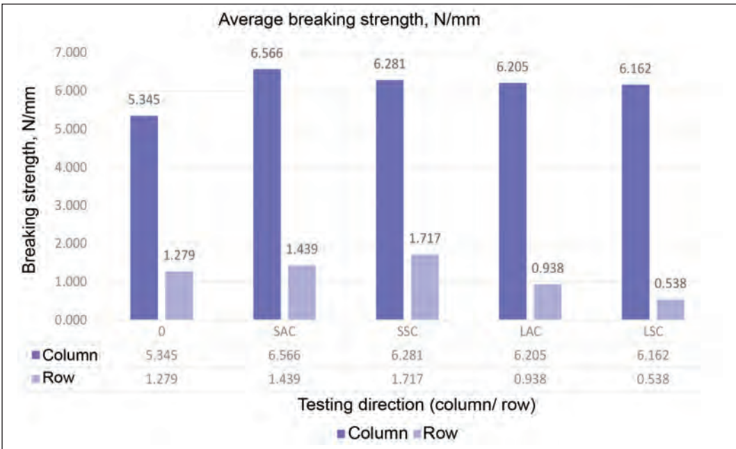
Fig. 5. Average breaking strength (N/mm) depending on the testing direction
