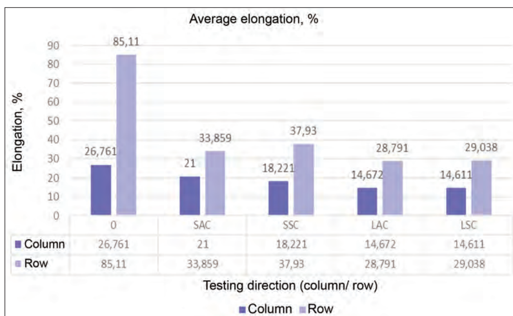
Fig. 4. Average elongation (%) depending on the testing direction
