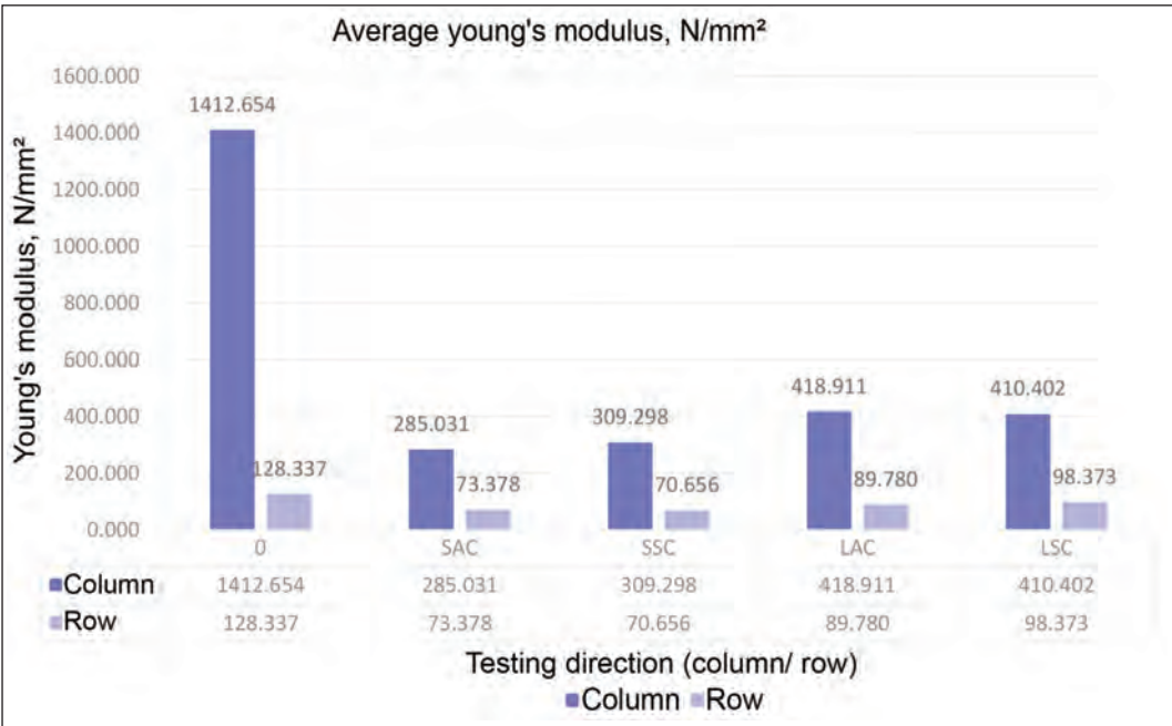
Fig. 7. Average Young's modulus (N/mm 2 ) depending on the testing direction
